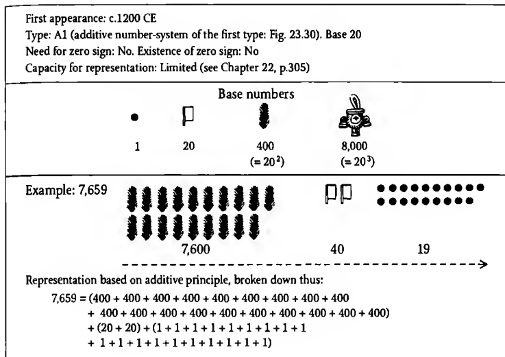
FIG. 23.6. Aztec number-system
