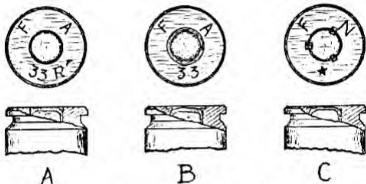
Variations in Primer Crimping.
