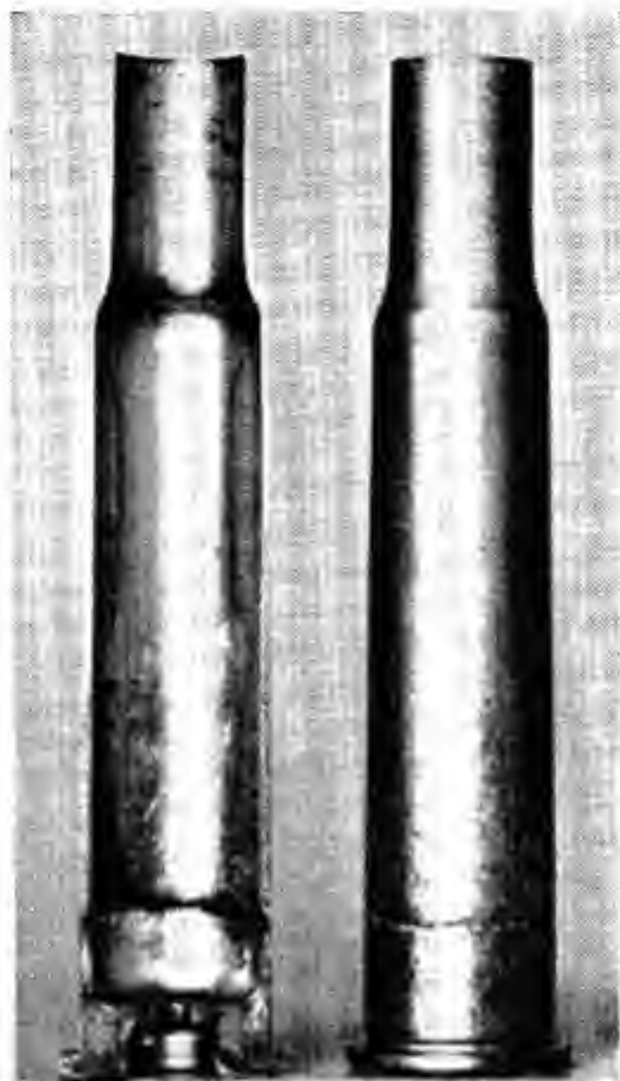
Halved sections of a .30/40 case which has been fired with a mercuric primer, then polished and etched. This case had split and stretched at the head, due to excess head space in the action.
