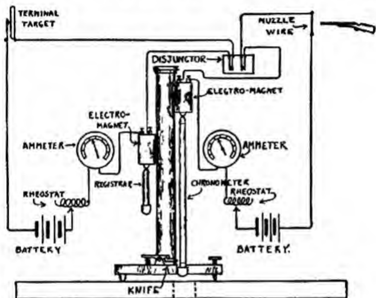
The Boulenger chronograph "hook-up" before the shot has been fired.
